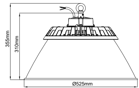
Tall Reflector
