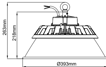
Universal Reflector
