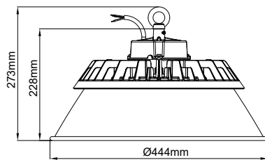
Universal Reflector
