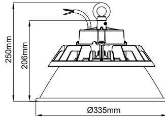
Universal Reflector
