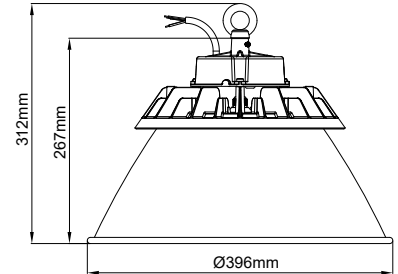
Tall Reflector
